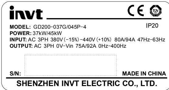
Fig 3-3 Name plate
