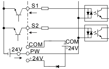
External power supply (NPN)
