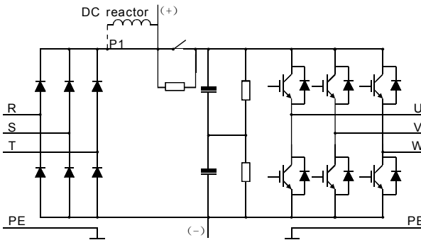
Diagram 3-2 The main circuit diagram (≥37kW)
