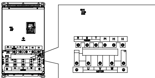
Fig 4-15 132~200kW terminals of main circuit
