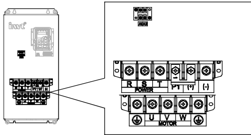
Fig 4-14 75~110kW terminals of main circuit
