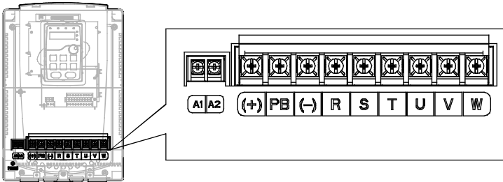
Fig 4-11 15~18kW terminals of main circuit
