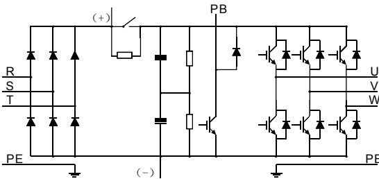
Diagram 3-1 The main circuit diagram (≤30kW)
