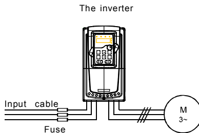
Fig 4-25 Fuse configuration
