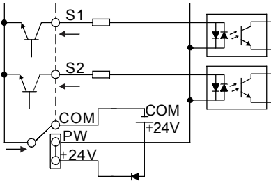
Internal power supply (NPN)
