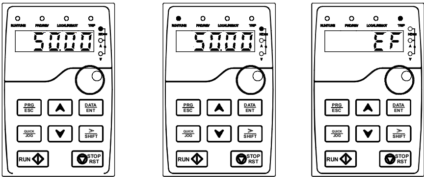
Fig 5-2 Displayed state
