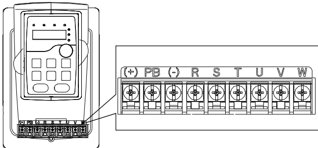
Fig 4-8 1.5~2.2 kW terminals of main circuit
