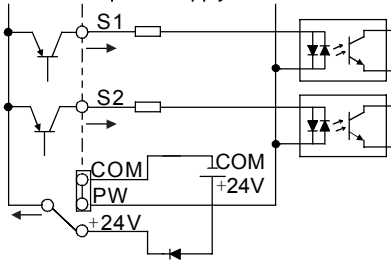
Internal power supply (PNP)
