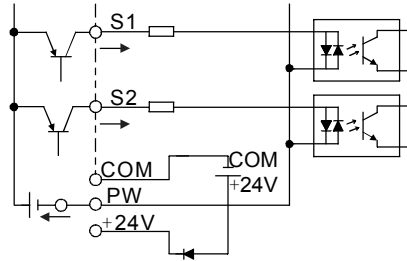
External power supply (PNP)
