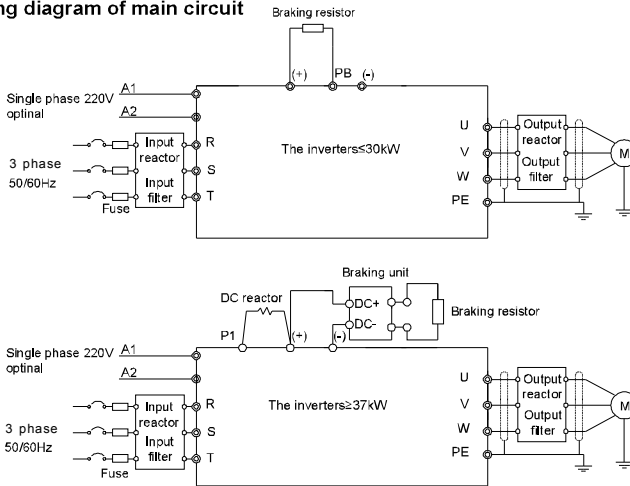
Fig 4-7 Wring diagram of main circuit
