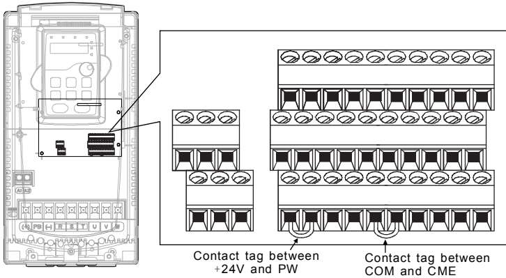
Fig 4-22 U-shaped contact tag
