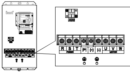
Fig 4-13 37~55 kW terminals of main circuit
