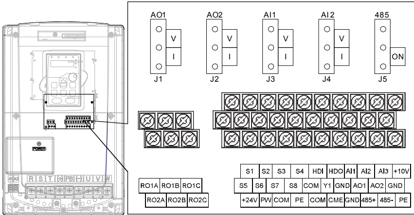
Fig 4-21 Terminals of control circuit
